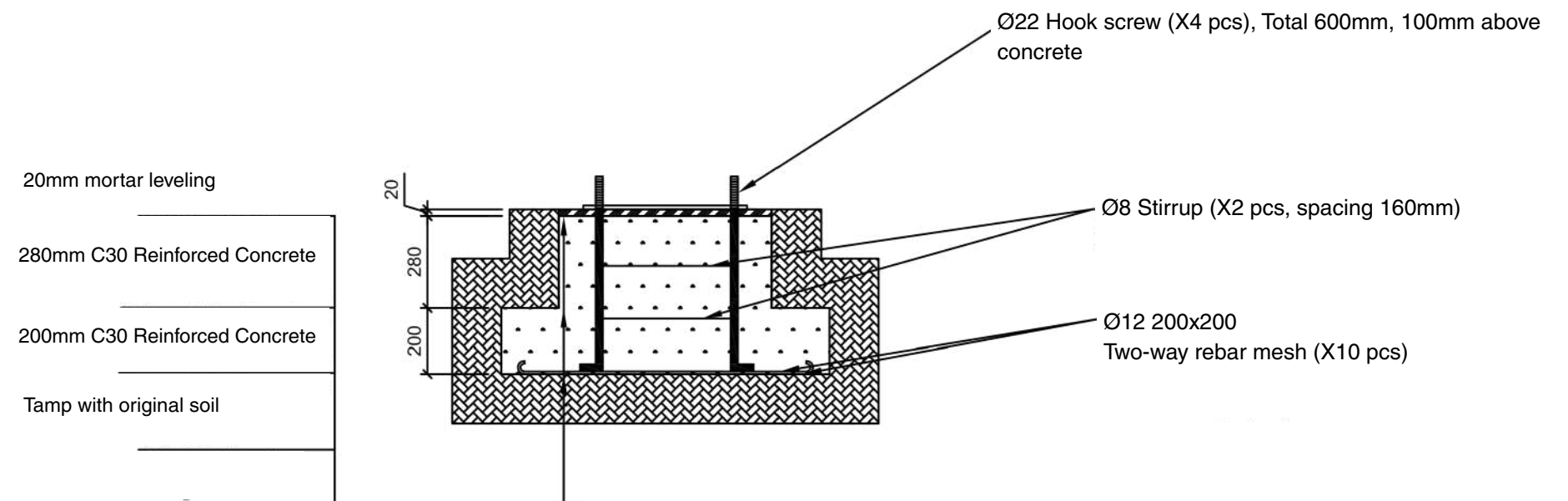
Base Vertical Cross-section
