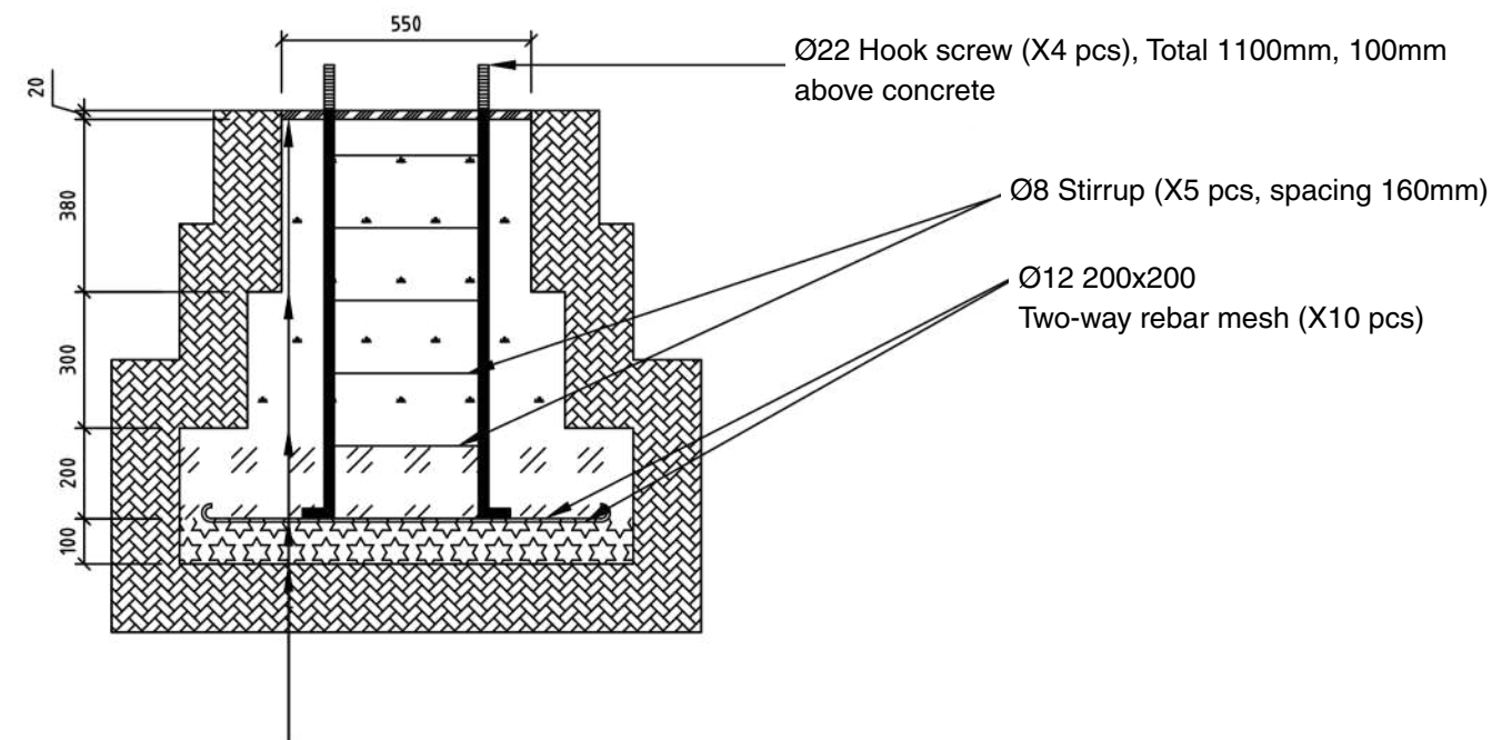
Base Vertical Cross-section
