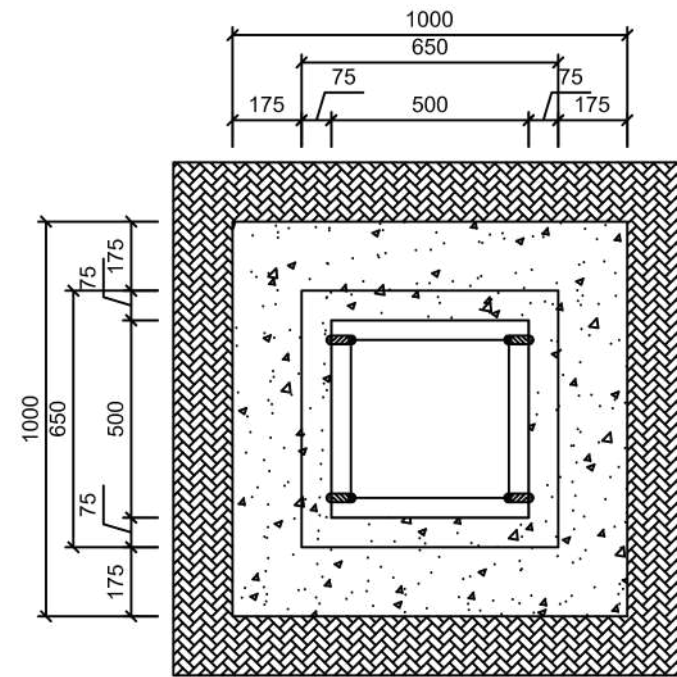
Base Vertical Cross-section
